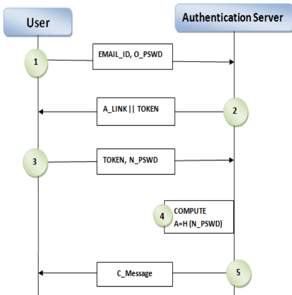
Figure 5: Password Change Process.
