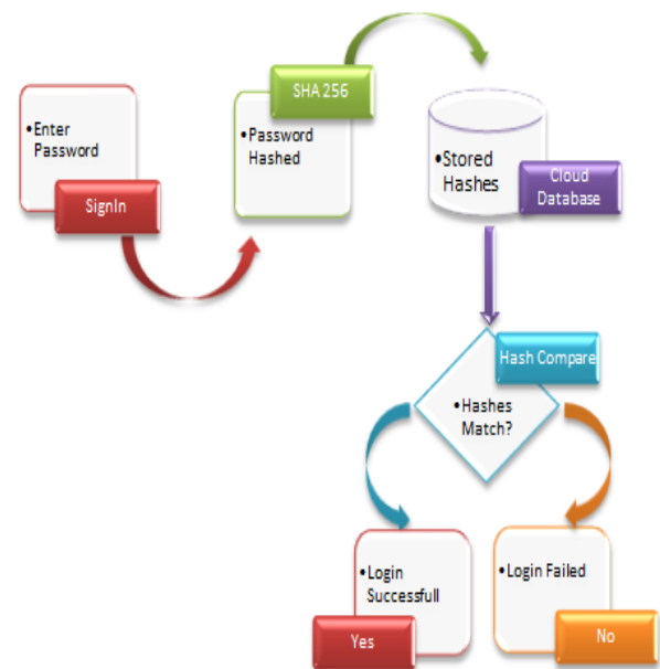
Fig 3b: Password Hashing and authentication based on hash.
