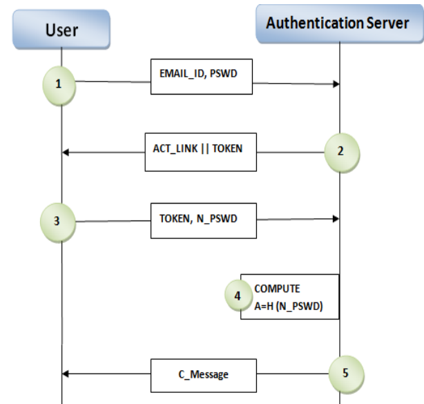
Fig 2: Registration Process
