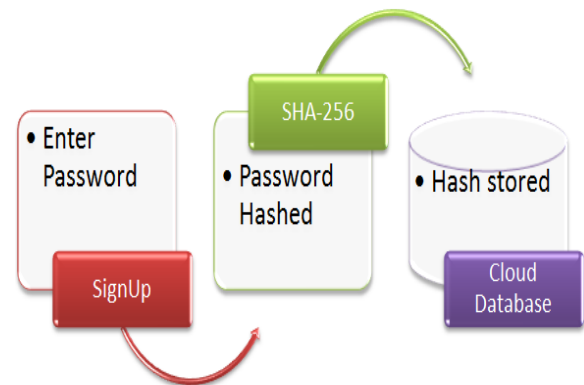
Fig 3a: Hashing of Password
